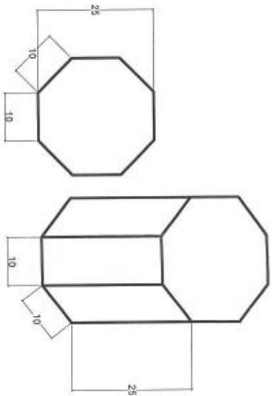
Detaliu sambure central
