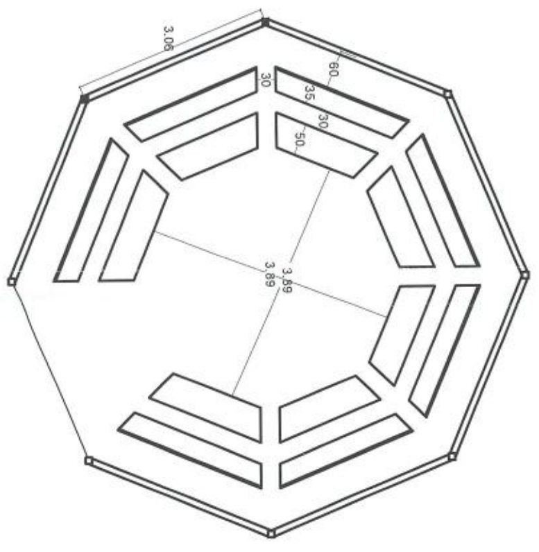
Varianta 2 - fara stalp central
