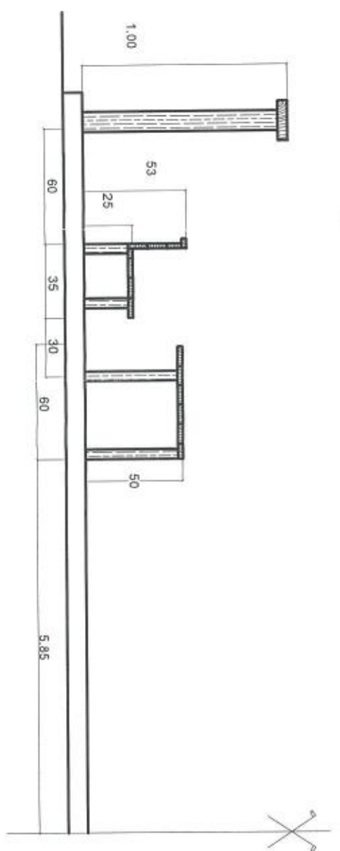
Varianta 2 - fara stalp central
