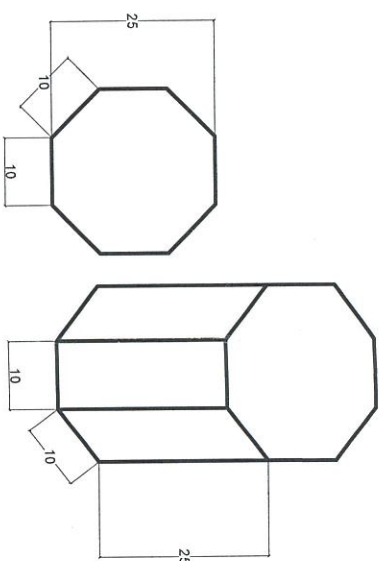
Detaliu sambure central
